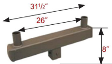
SQUARE VERTICAL TENON 2 @ 180° S5VT2S18BZ
