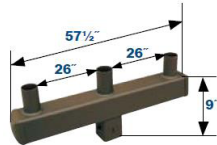
SQUARE VERTICAL TENON 3 @ 180° S5VT3S18BZ
