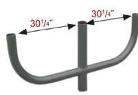
ROUND BULLHORN 3 @ 180° BH3RBZ
