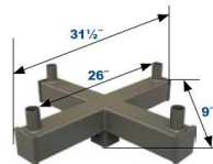
SQUARE VERTICAL TENON 4 @ 90° S5VT4S90BZ
