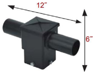
SQUARE HORIZONTAL TENON 2 @ 180° S5HT218BZ
